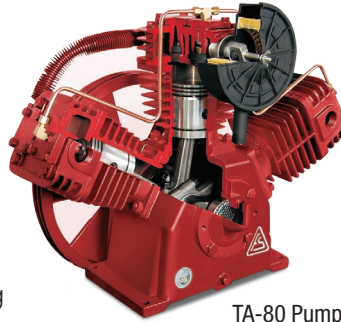
TA-80 Pump
